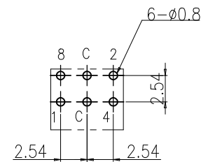
P.C.B DIMENSION (Top View)
